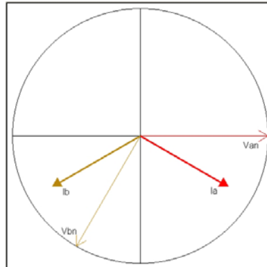
30° Lag (0.866 PF)
